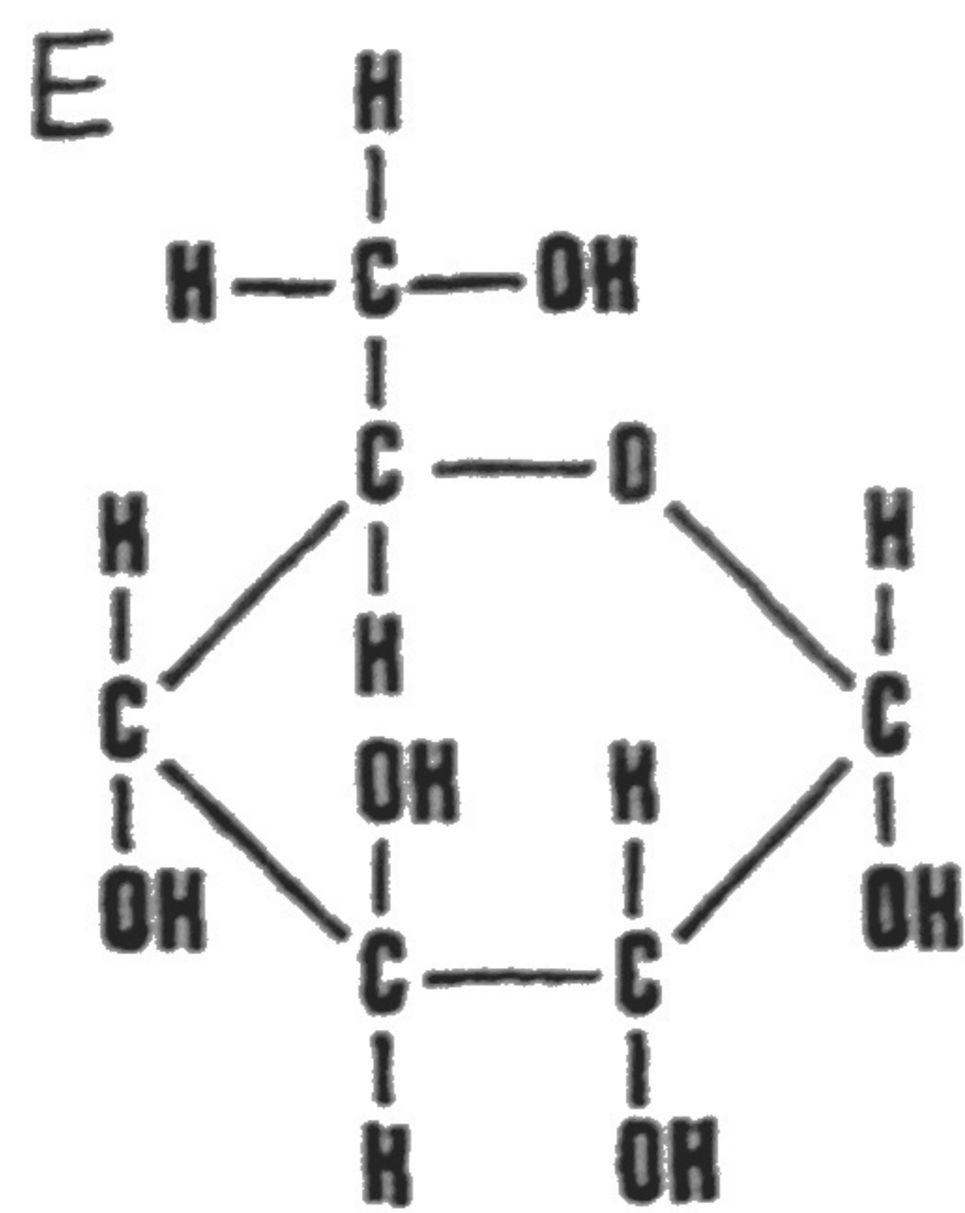
Glucose
