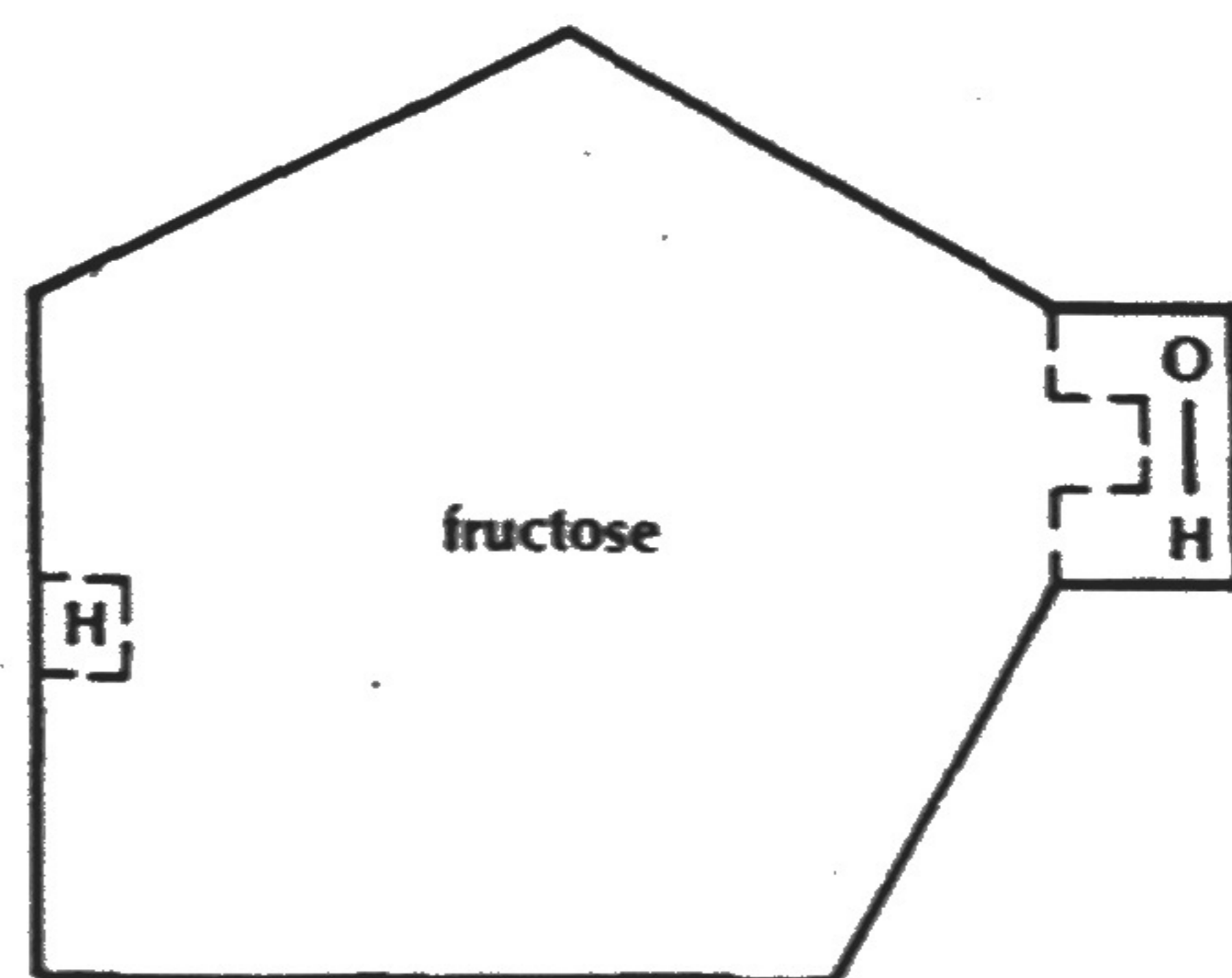
model of fructose
